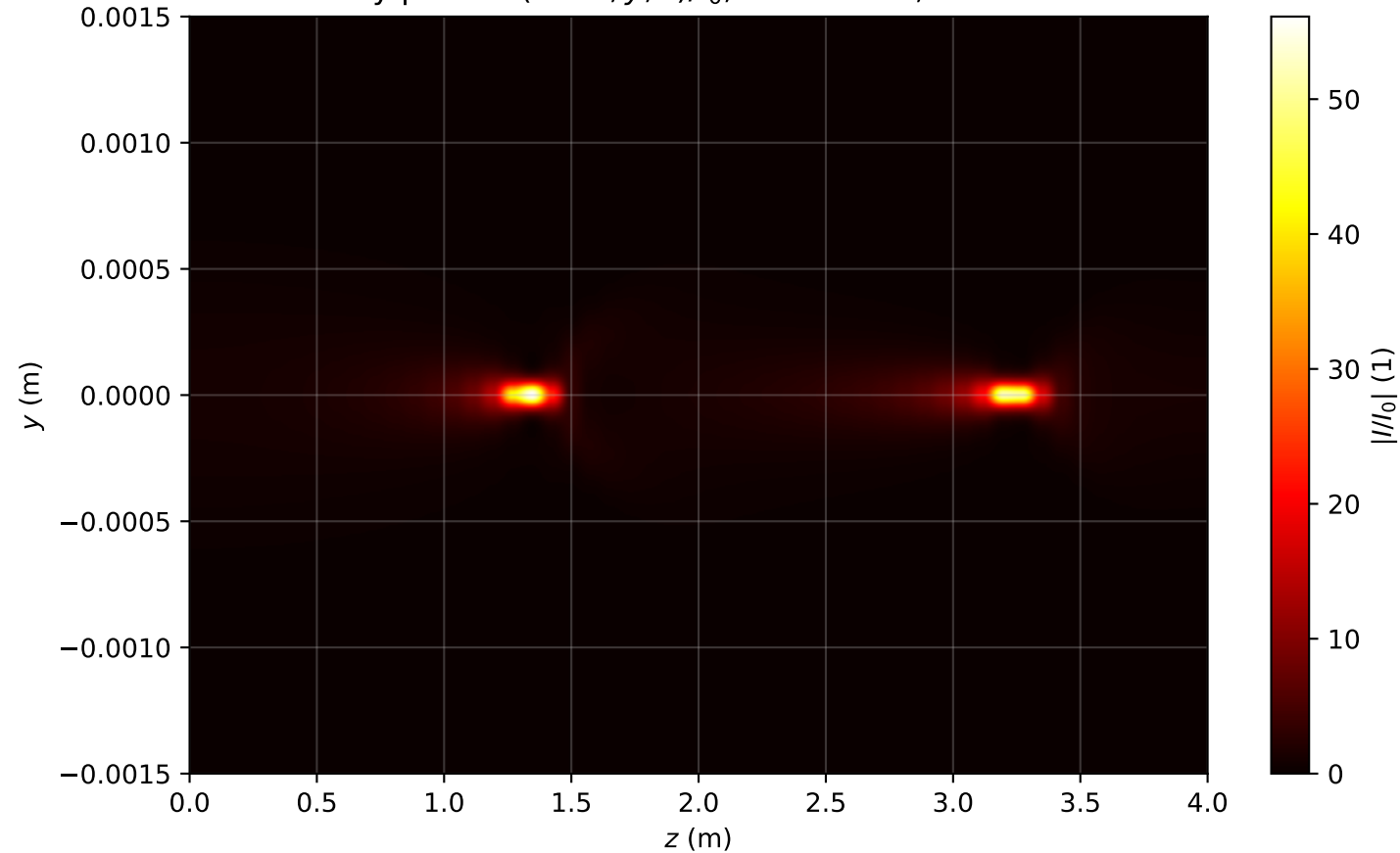
Intensity profile I(x=0, y, z)/I_0 , P_{in}=1.8P_{cr} , artificial time
